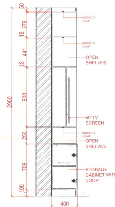
Sectional Details
